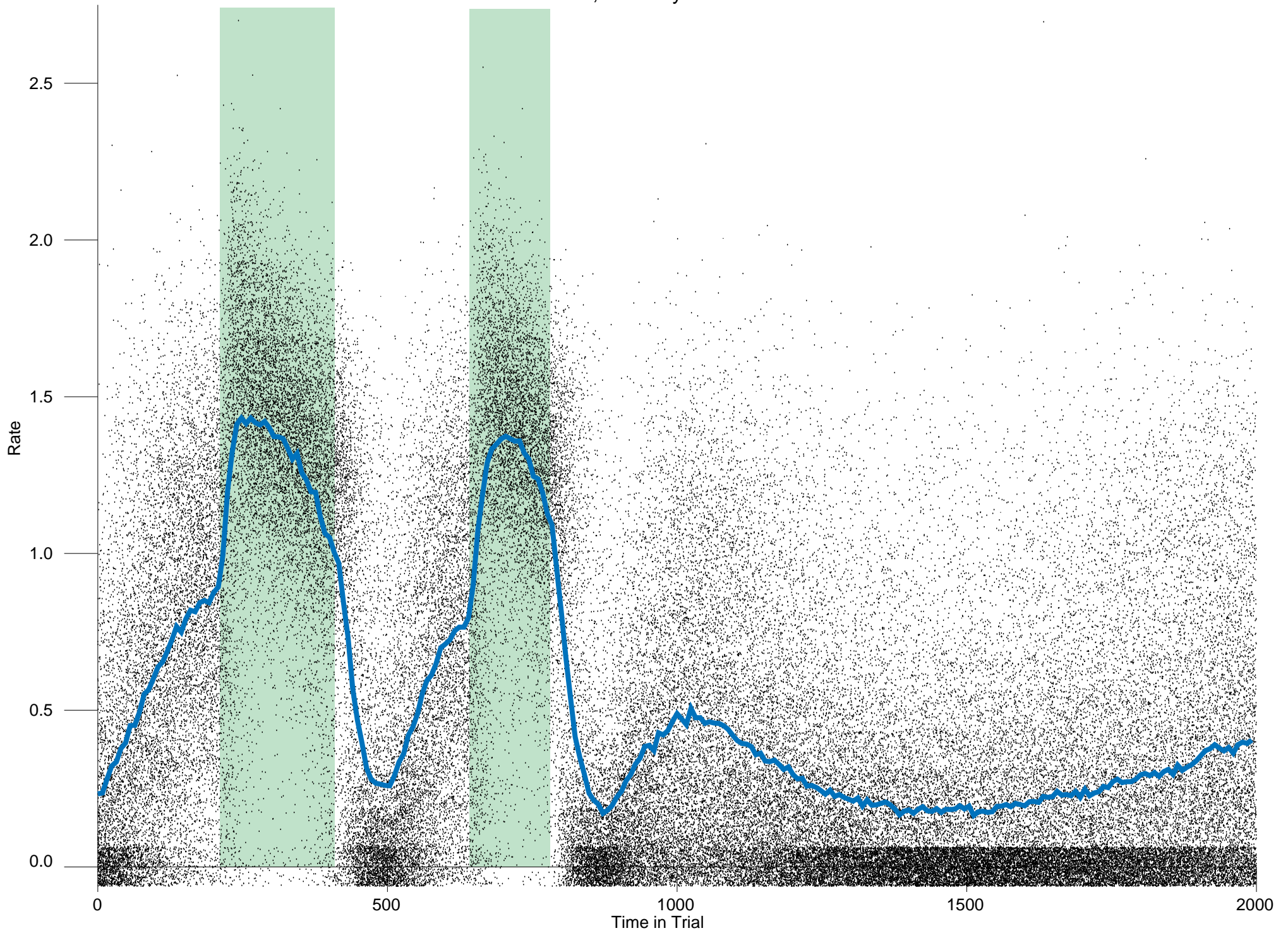
Bird 589: 8.0 Sec bins, 100 Days End: 11/25/97
